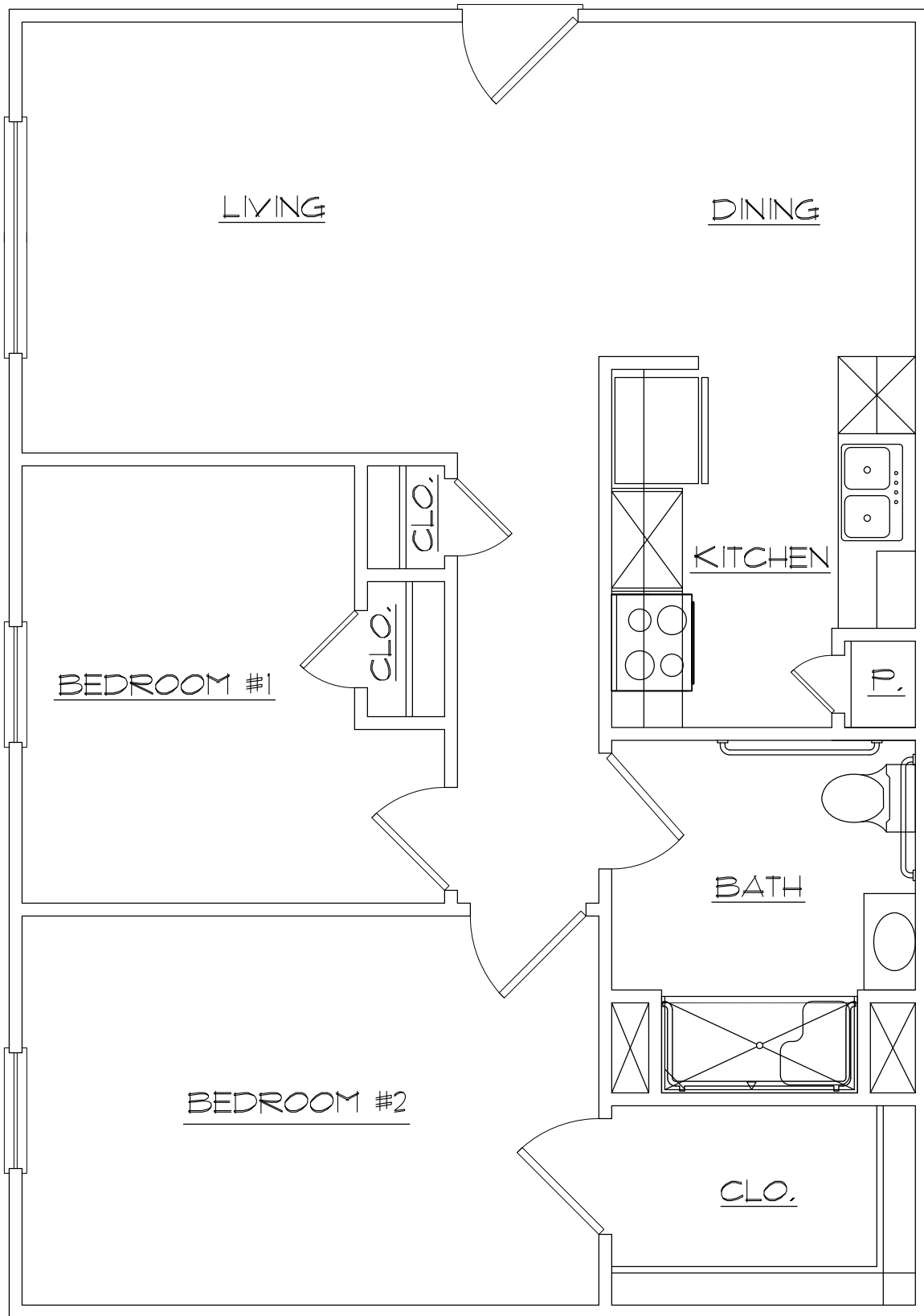
SAN GABRIEL APARTMENTS UNIT FLOOR PLAN B1 ACCESSIBLE 2 BEDROOM 1 BATH APPROX. 800 SQ. FT.
